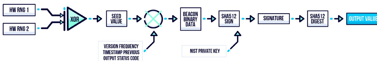
Fig 12: NIST Randomness Beacon Process 12
