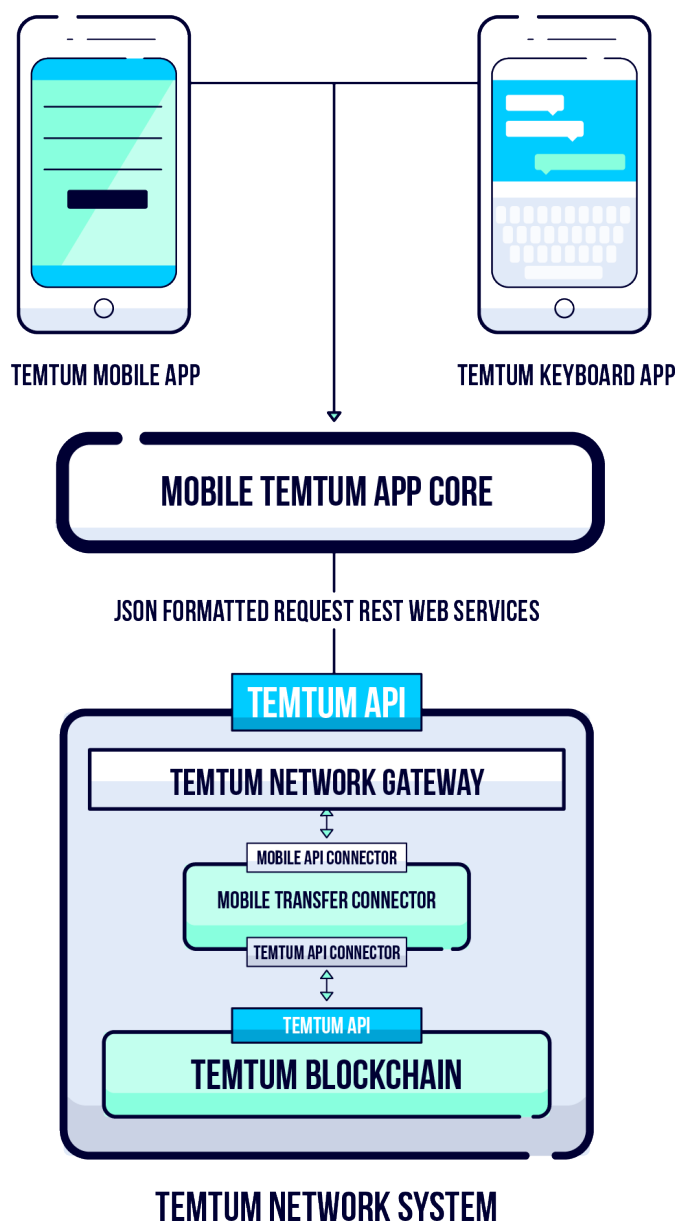
Fig 33: Mobile apps API integration
