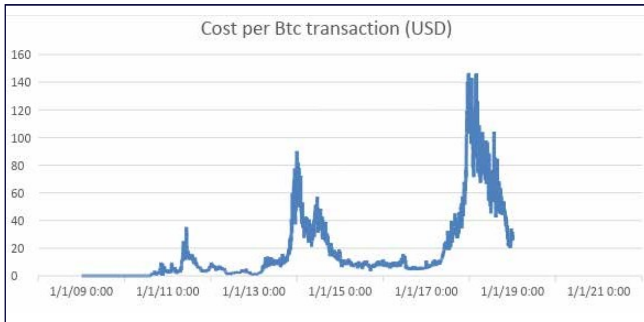
Fig 37: Cost per Bitcoin transaction
