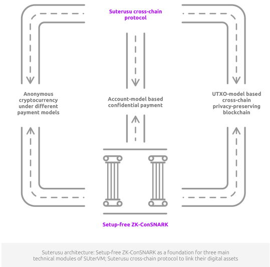
Fig. 2. Suterusu architecture
