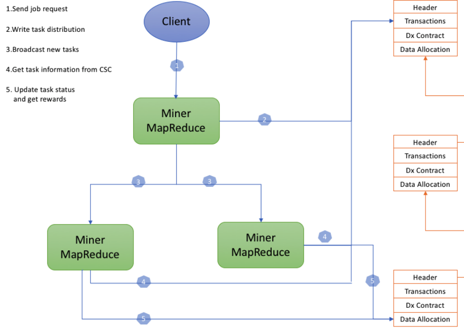
Figure 4.3: Illustration of Computing Side Chain (CSC) Overview.
