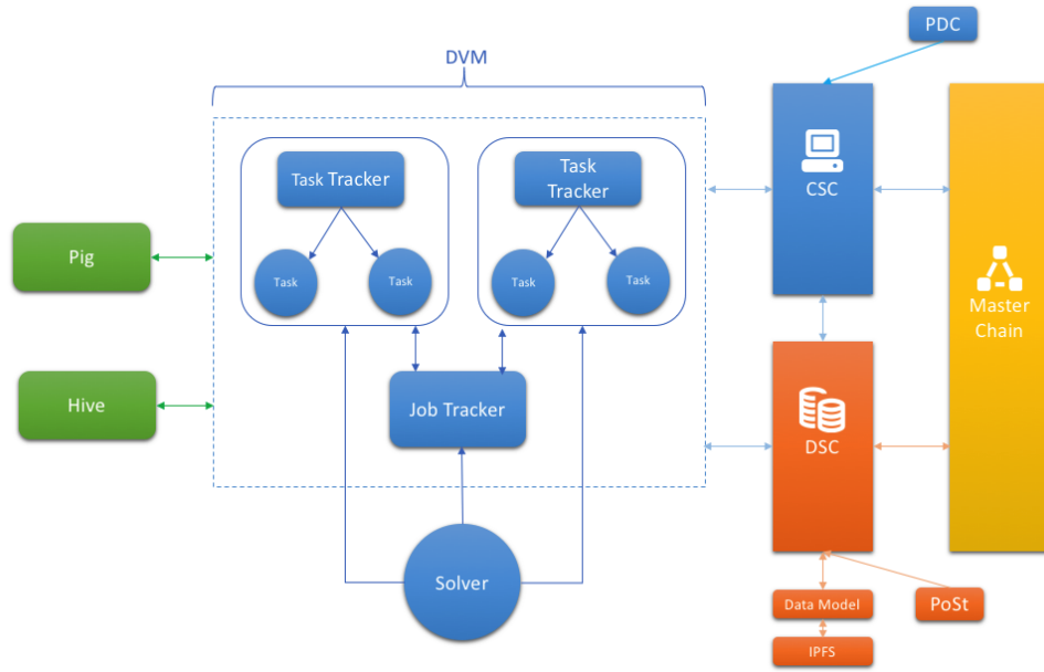
Figure 3.1: Illustration of High-level DxChain Network Infrastructure.
