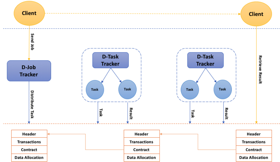
Figure 7.2: Illustration of map-reduce process in DxChain Network.
