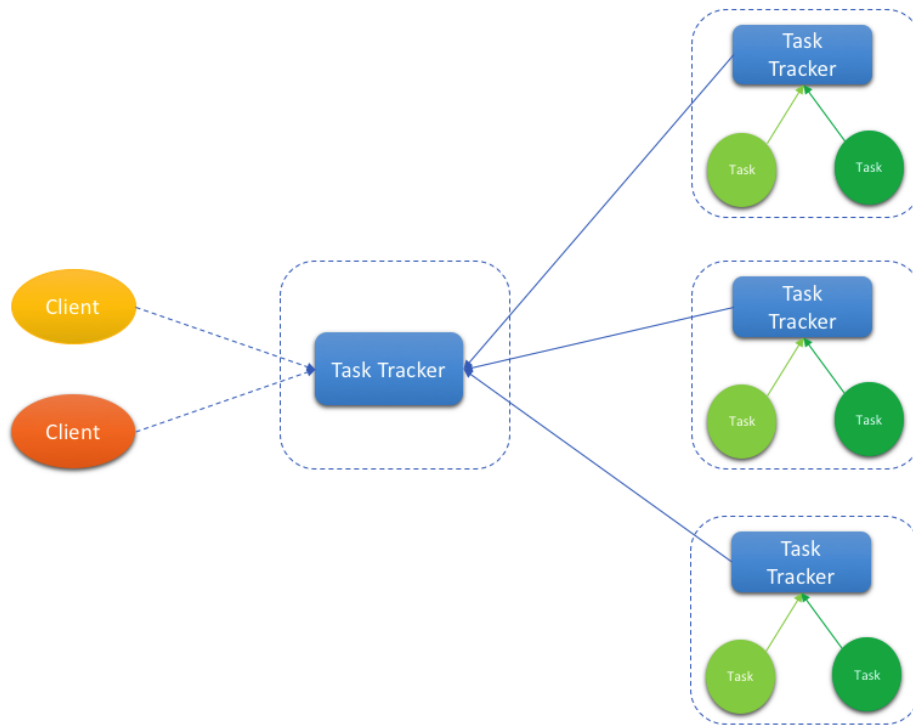
Figure 7.1: Illustration of general map-reduce process.
