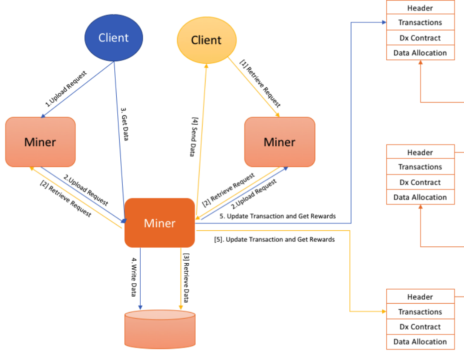
Figure 4.2: Illustration of Data Side Chain (DSC) Overview.
