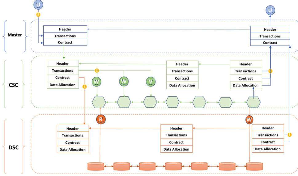
Figure 4.4: Illustration of DxChain Cross Chain Communication Protocol.
