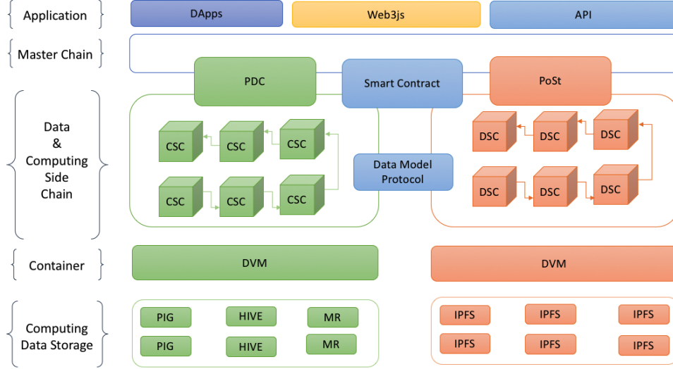
Figure 4.1: Illustration of DxChain Network Design Overview.
